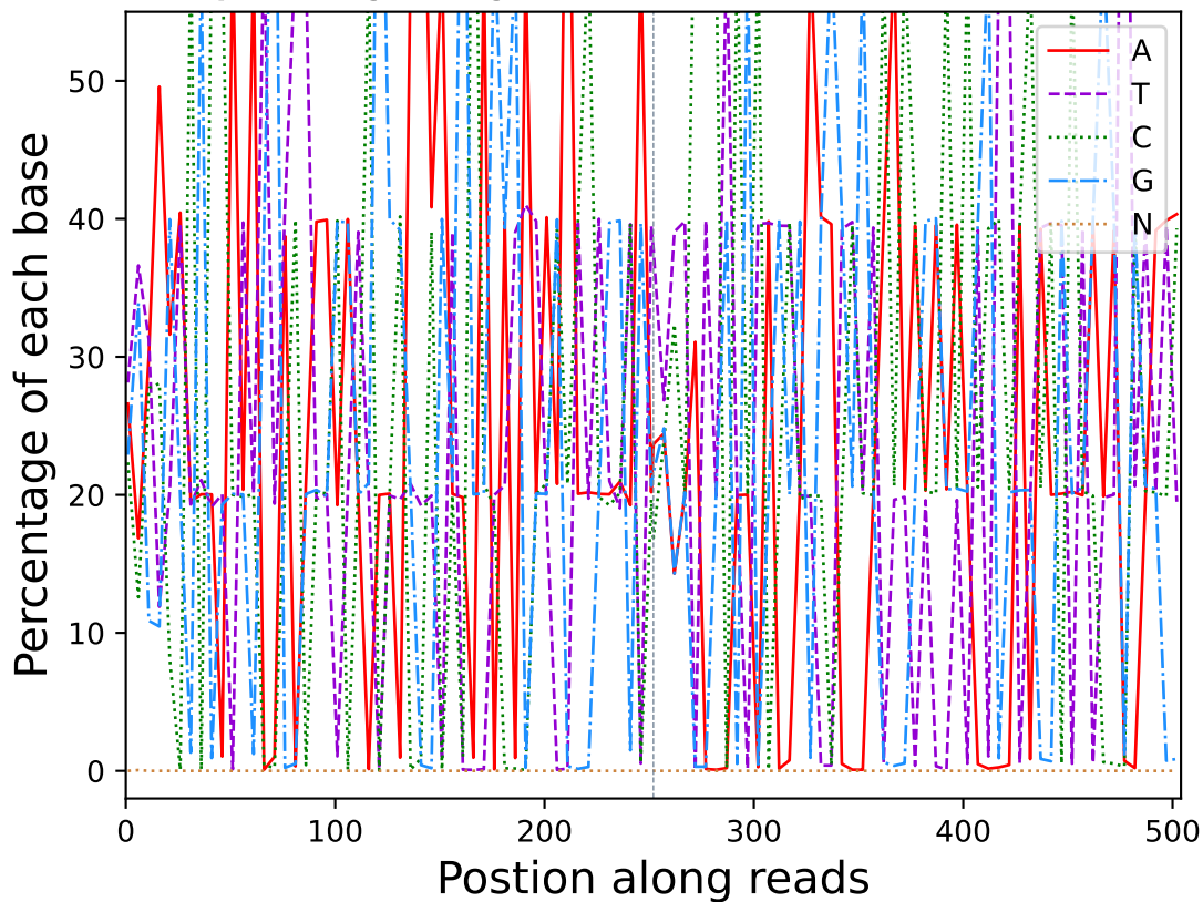
Base percentage along reads (R10701)
